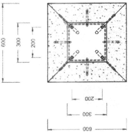
TOP VIEW SCALE 1 : 15
